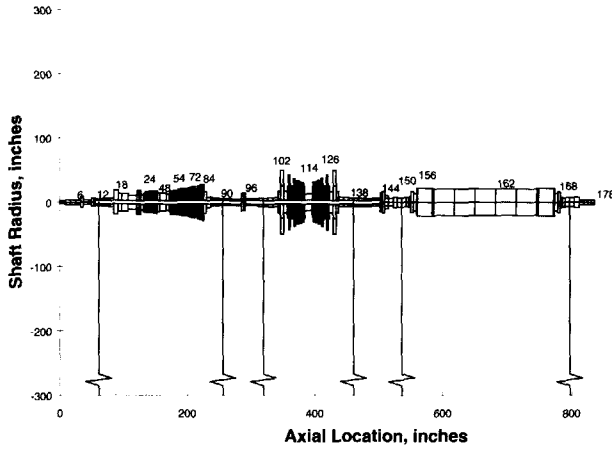
Figure 4. Turbine Generator Rotor Modelled from Left to Right.
