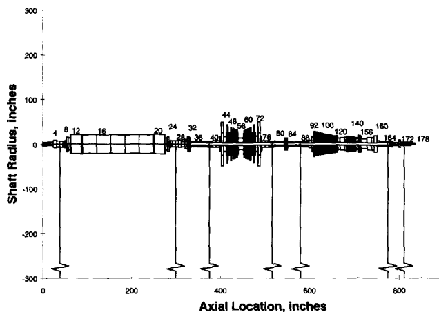
Figure 15. Rotor Model with Steady Bearing at Station #173.
