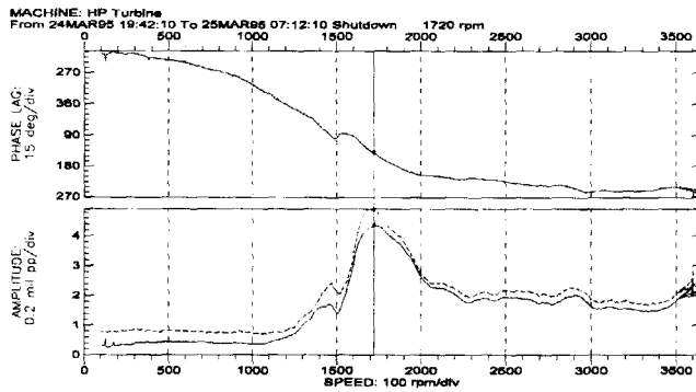
Figure 6. Cooldown Data at #2 Bearing Location.
