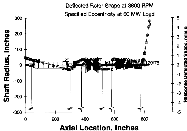
Figure 26. Deflected Rotor Shape.
