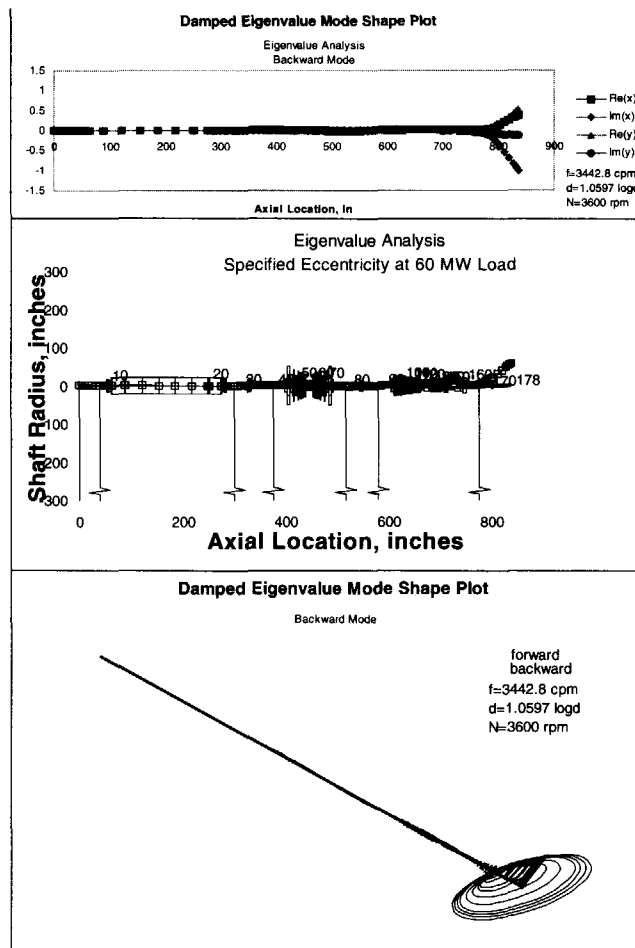
Figure 25. Eigen Analysis Predicting the Backward Mode.
